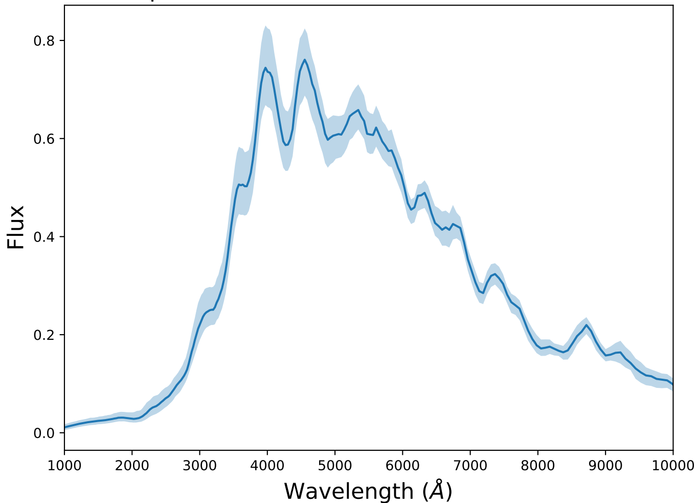
Spectrum 10 for transient SNIax at z=1.10
